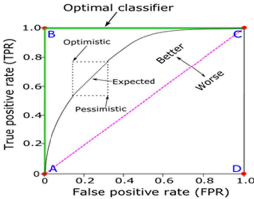
Fig 3: Basic ROC Curve showing important Points
