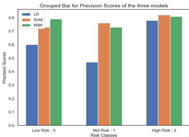
Fig 143: Group bar chart showing precision scores obtained from the three ML Models
