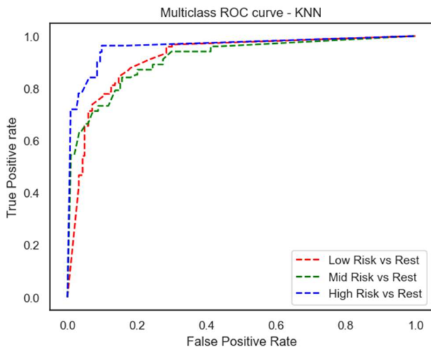
Fig 12: Multiclass ROC Curve showing a class vs the rest using the KNN Model
