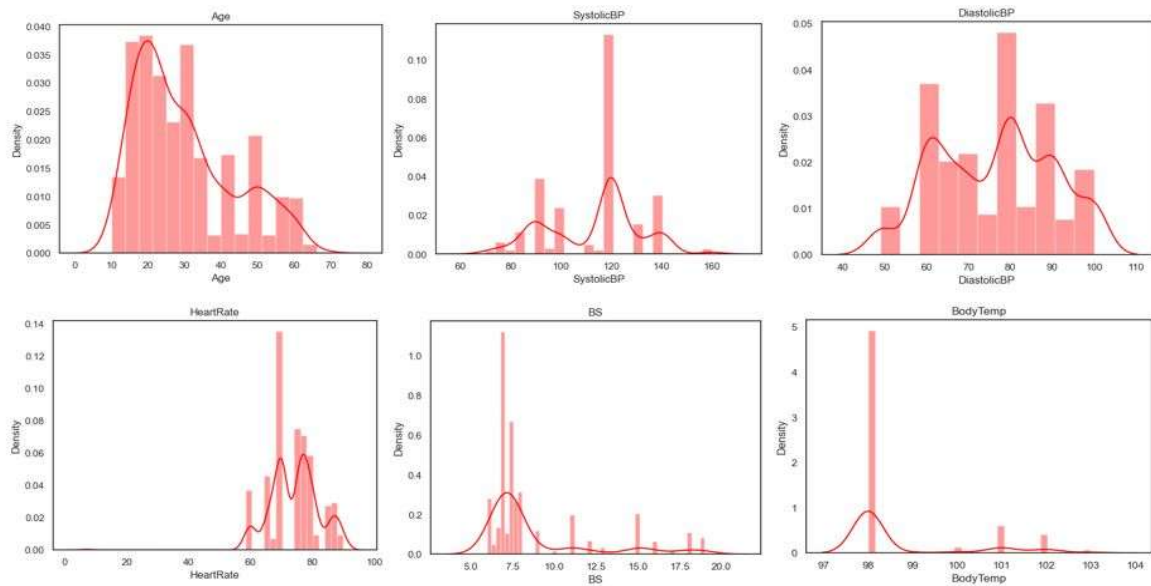
Fig 1: An explorative data analysis of the independent features within the dataset
