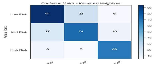
Fig 10: Confusion matrix obtained using KNN
