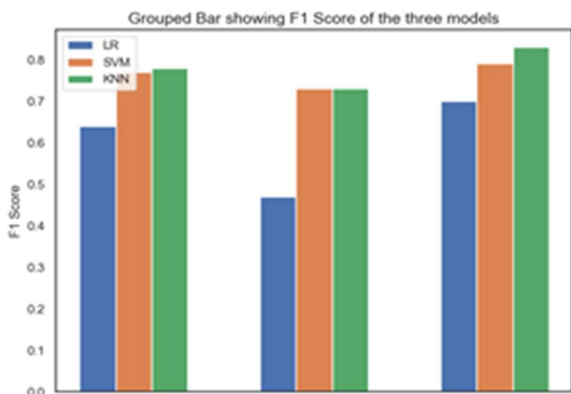
Fig 16: Group bar chart showing F1 scores obtained from the three ML Models
