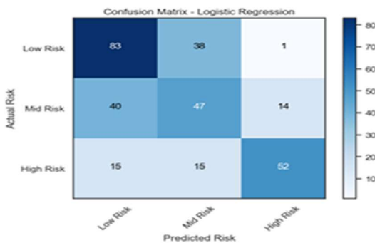
Fig 4: Confusion matrix obtained using LR
