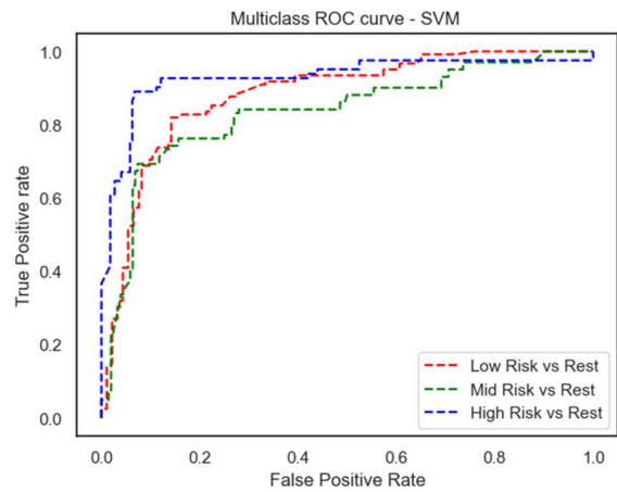
Fig 9: Multiclass ROC Curve showing a class vs the rest using the SVM Model
