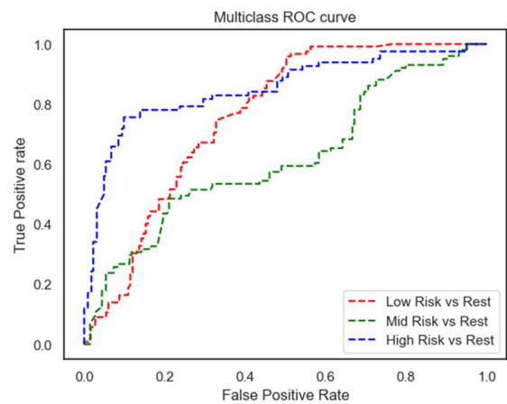
Fig 6: Multiclass ROC Curve showing a class vs the rest
