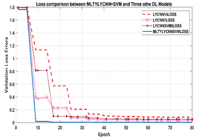
Figure 4. Validation Loss Comparison between the proposed MLTYLY CNN and Three Deep Learning Model Architectures
